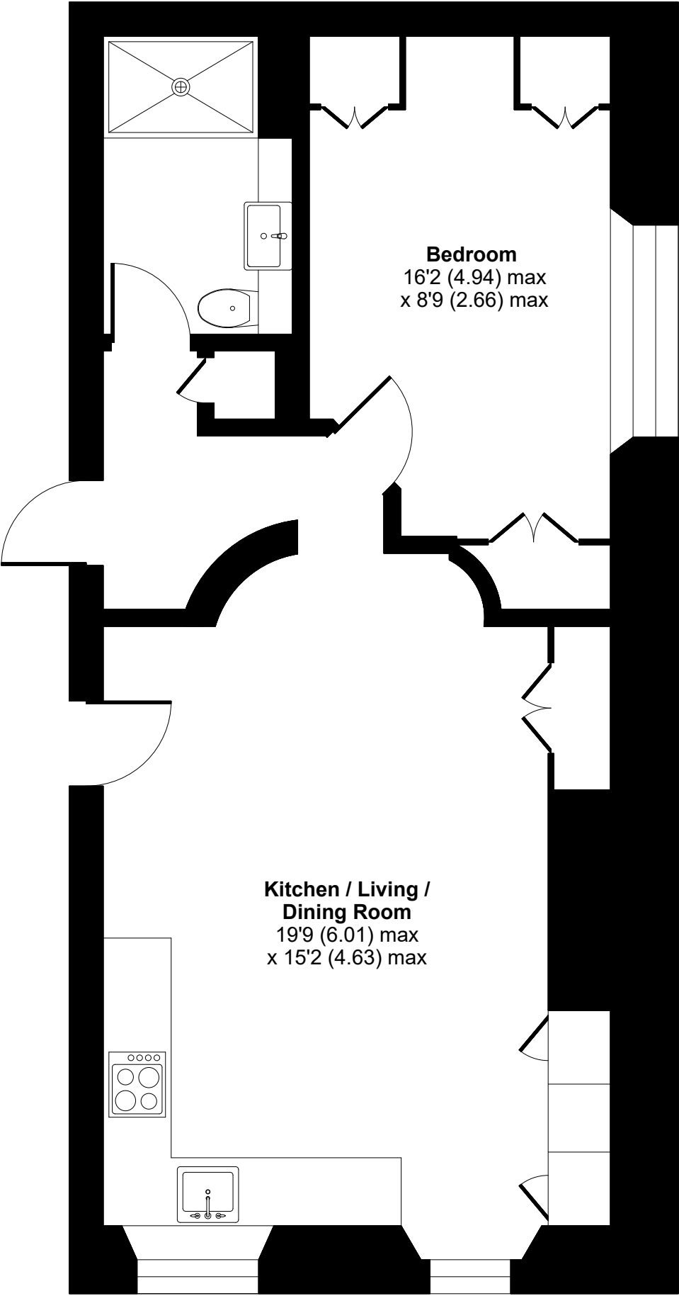
GROUND FLOOR
